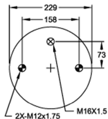
3705 BEAD PLATE
